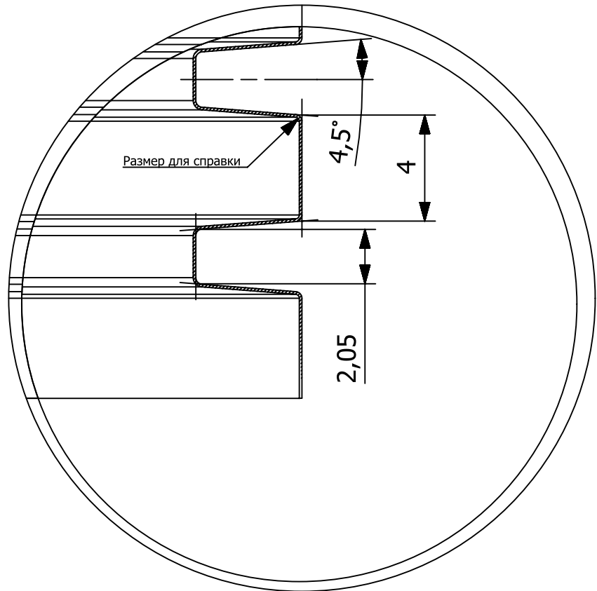
DETAIL A SCALE 5:1
